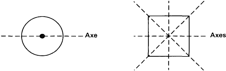
FIGURE 20-1 Divers types de symétries.
