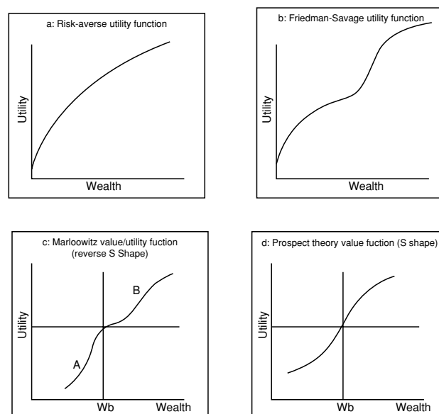
Figure 26.2. Alternative shapes of the utility/value function
