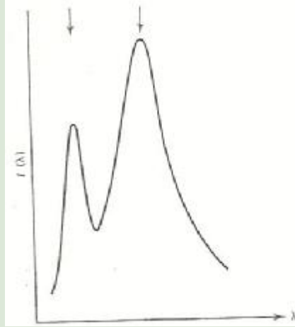
Figure 1-6. The spectrum of radiation scattered by carbon, showing the unmodified line at 0.7078 Å on the left and the shifted line at 0.7314 Å on the right. The former is the wave-length of the primary radiation.
