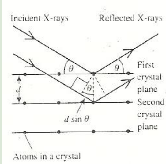
Figure 1-8 the scattering of X-rays by crystal planes when the angle \theta between the scattered X-rays and the crystal plane equals the angle between the incident X-rays and the plane.
