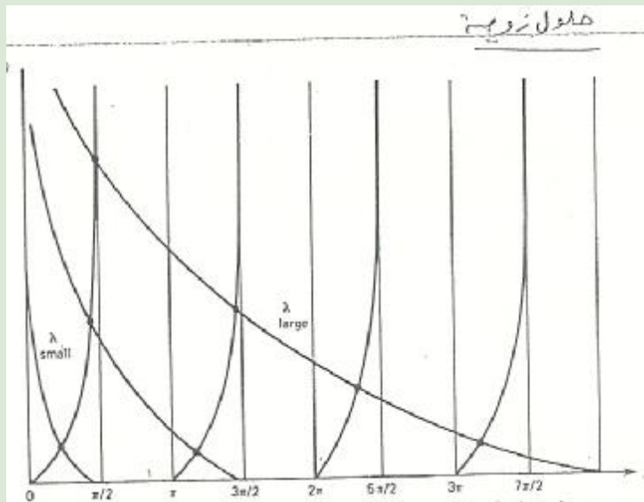
Figure 5-11. Location of discrete eigenvalues for even solutions in square well. The rising curves represent \tan y ; the falling curves are \sqrt{l - y^2/y} for different values of l
