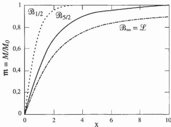
Figure A 6.3 - Allure des courbes \mathfrak{B}_{1/2}(x) , \mathfrak{B}_{5/2}(x) et \mathcal{L}(x)
