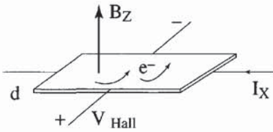
Figure 14.1 - Tension de Hall V_y
