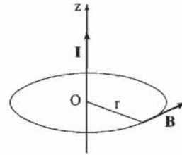
Figure 2.3 - Courant filiforme
