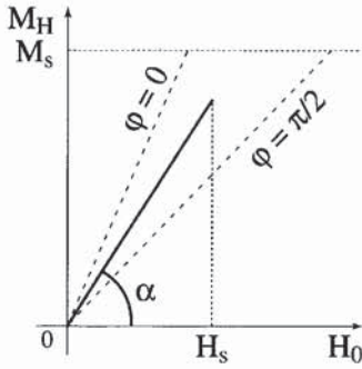
Figure 5.41 - Processus d'aimantation ( H_0 < H_s )
