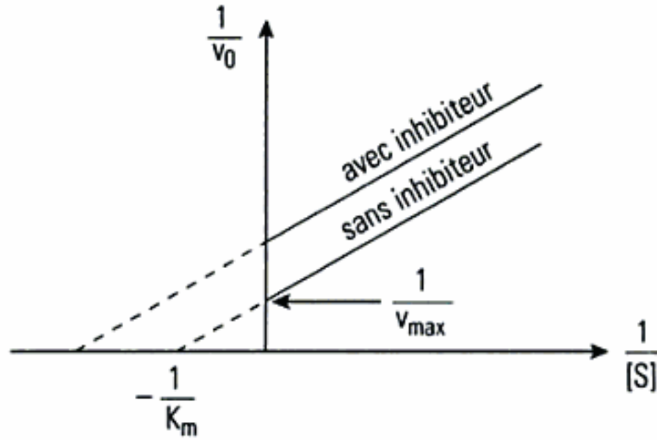
Fig. 3 – Inhibition irréversible.
