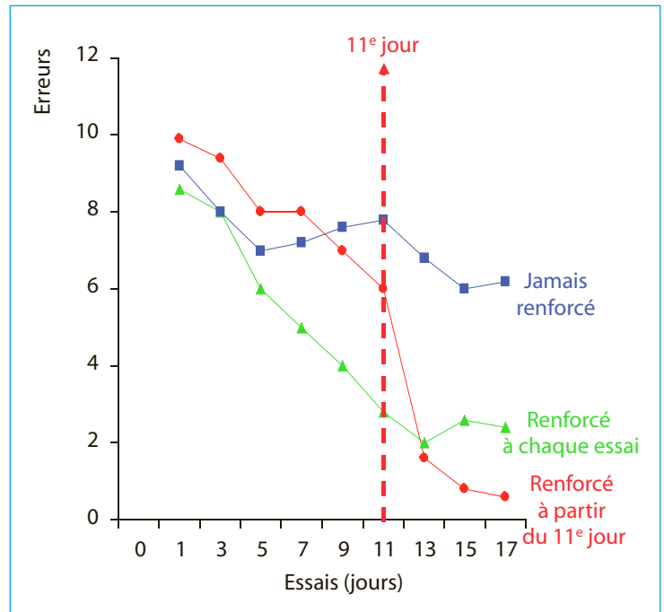
Figure 4.20 – Apprentissage latent.
